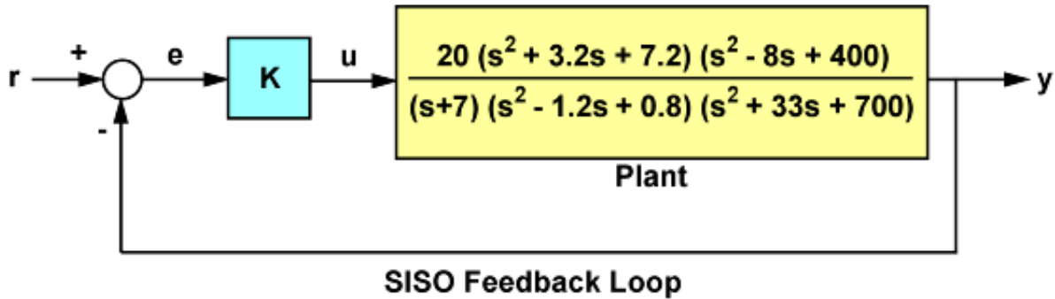
Figure 2: Feedback Loop with Multiple Phase Crossovers
